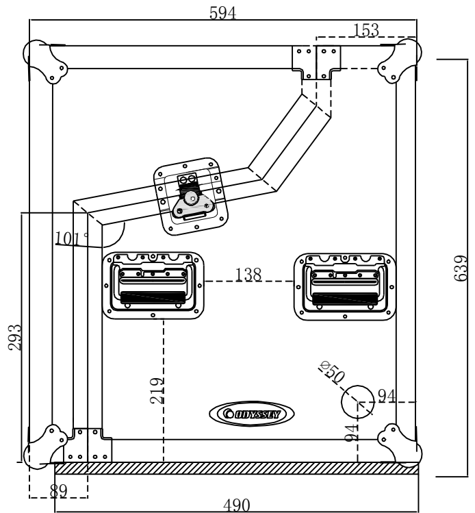
Side View
